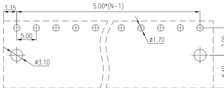
PCB LAYOUT
